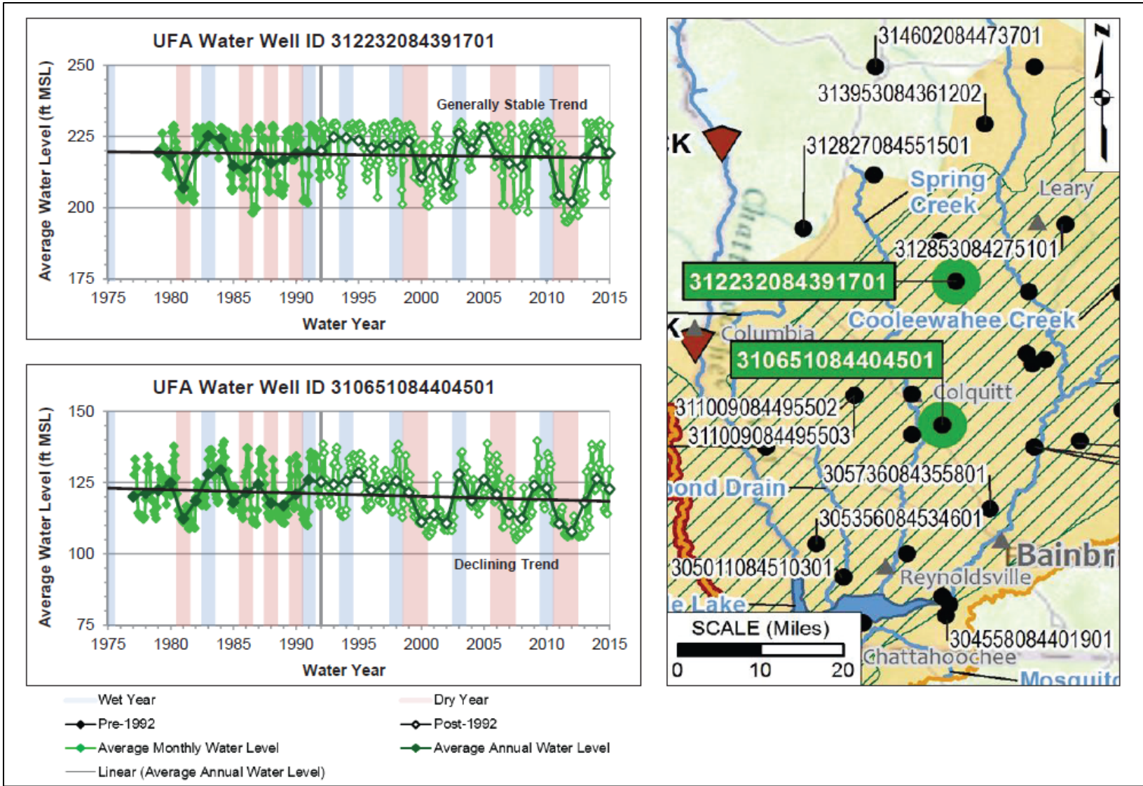
Panday Demo. 35c — Hydrographs for Select UFA Water Wells
