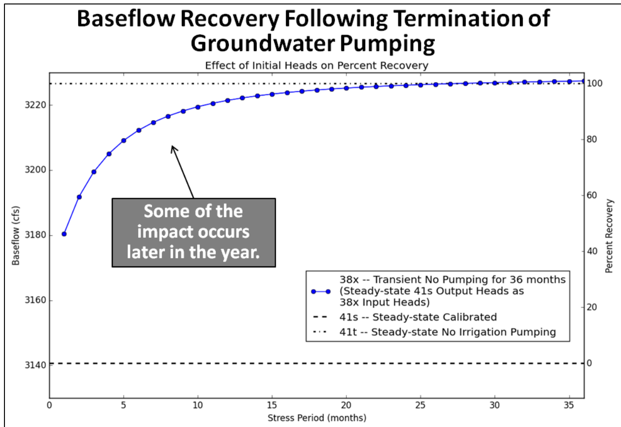
Panday Demo. 23 — Source: Panday Expert Report (GX-0873), 20 May 2016, Figure 5-7.
