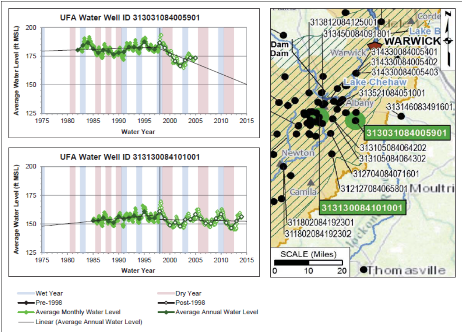
Panday Demo. 41f — Modified from Panday Expert Report (GX-0873), 20 May 2016, Fig.C-24. Data was obtained from the USGS (JX-128).
