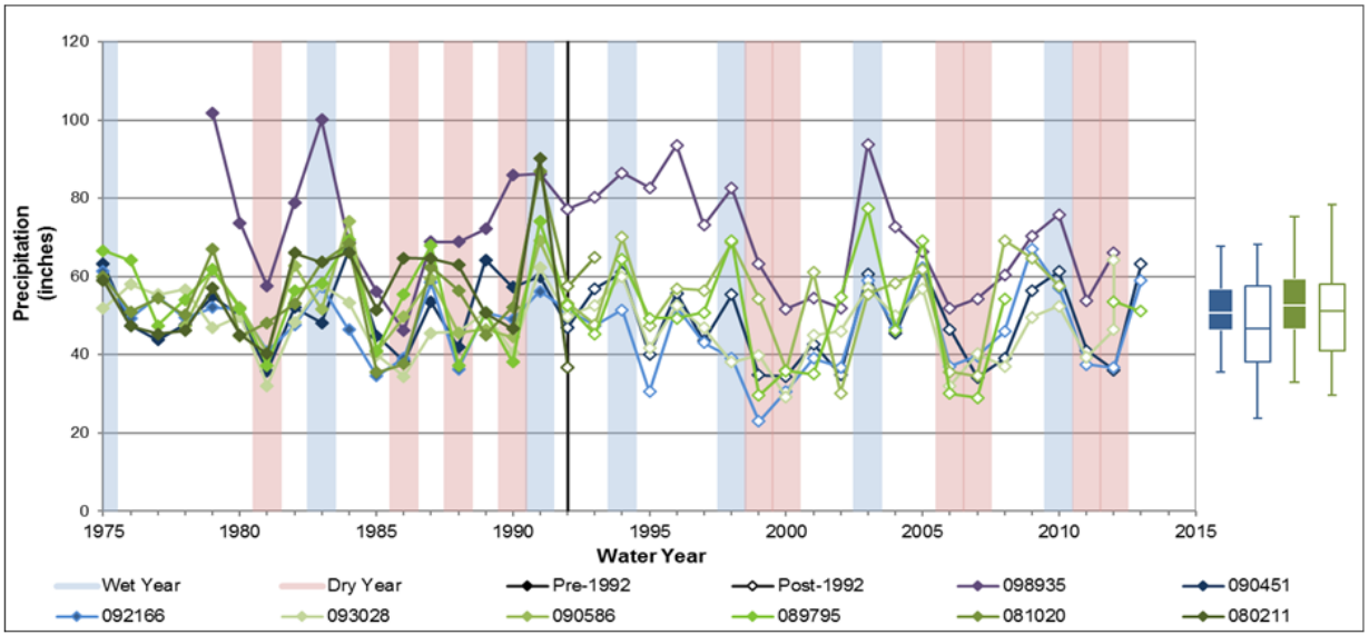
Summary Statistics
