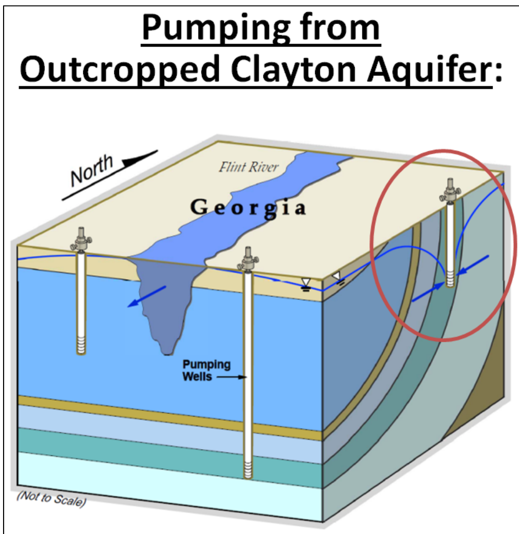
Panday Demo. 27 — Modified from Panday Expert Report (GX-0873), 20 May 2016, Fig. D-2.
