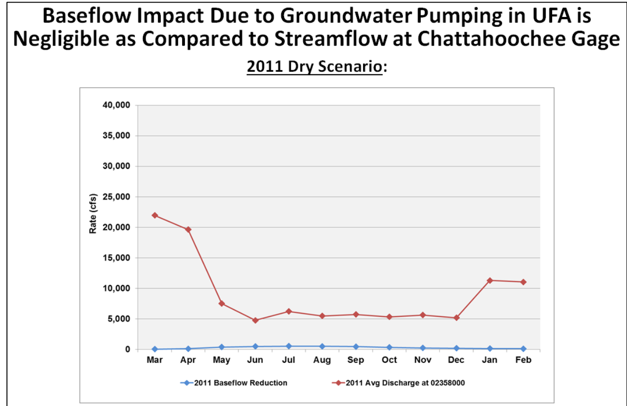
Panday Demo. 15 — Created from data in Panday Expert Report (GX-0873), 20 May 2016, Revised Fig. E-9. Flow data from Chattahoochee gage was obtained from the USGS (JX-128).
