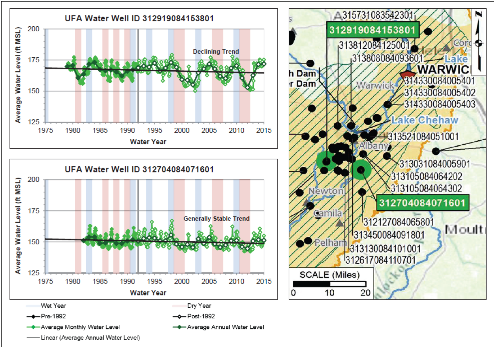
Panday Demo. 35h — Hydrographs for Select UFA Water Wells
