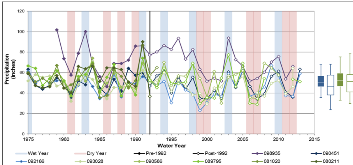
Summary Statistics
