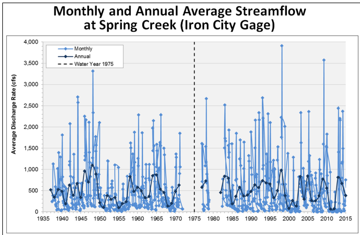
Panday Demo. 44 — Panday Expert Report (GX-0873), 20 May 2016, Fig. F-5. Data was obtained from the USGS (JX-128).
